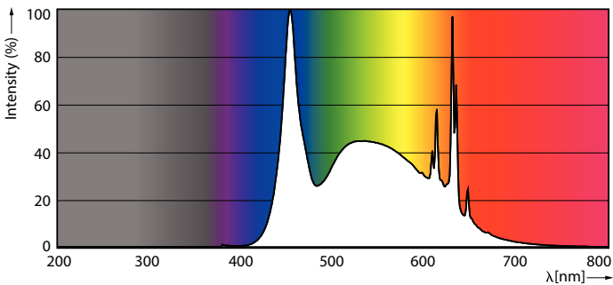
Spectral Power Distribution Colour - LEDspot GU10 6-50W D 865 35D 120V 1PF/6
