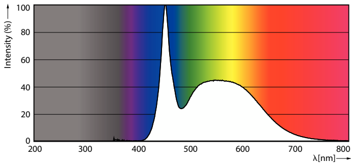
Spectral Power Distribution Colour - LEDBulb 22W E27 6500K W A25 1PF/6 MX
