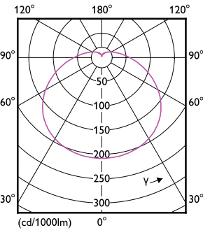
Light Distribution Diagram - LEDBulb 22W E27 6500K W A25 1PF/6 MX
