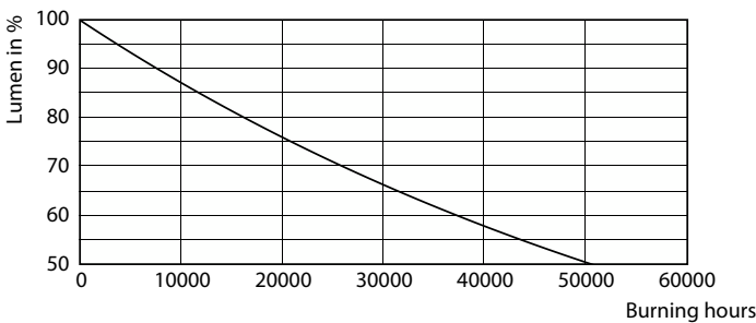
Lumen Maintenance Diagram - LEDBulb 22W E27 6500K W A25 1PF/6 MX
